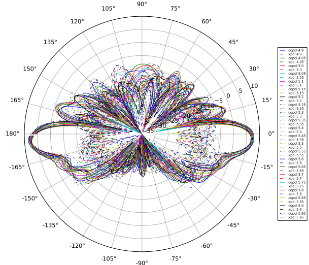
Omni Elevation
