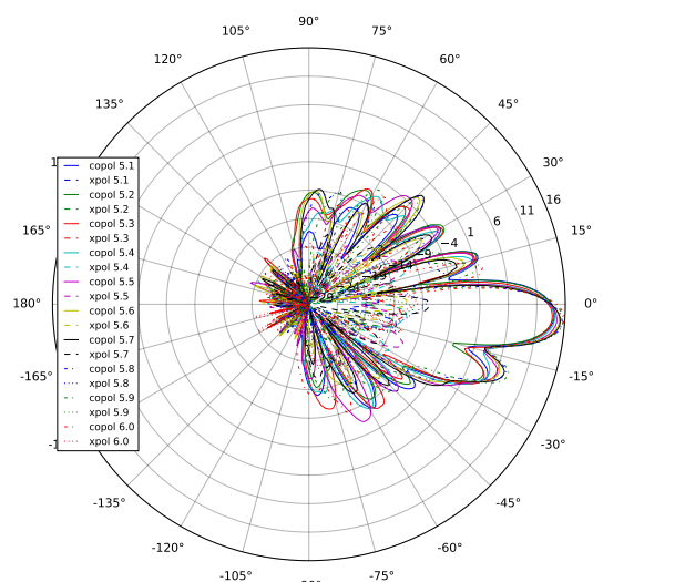
Sector Elevation
